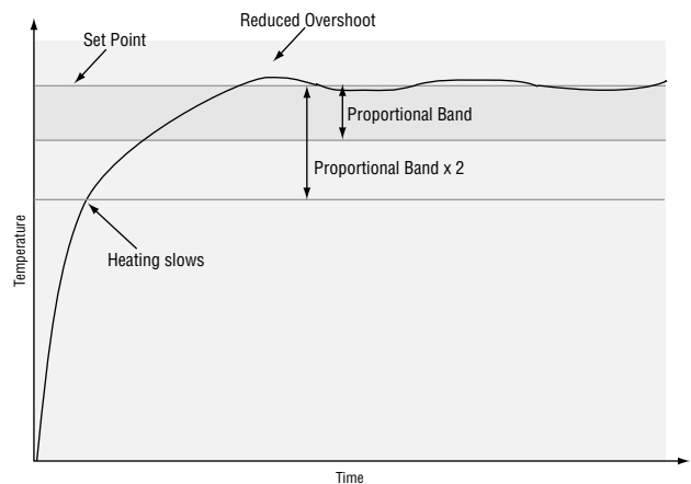
Figure 6.5b — PID Control.
